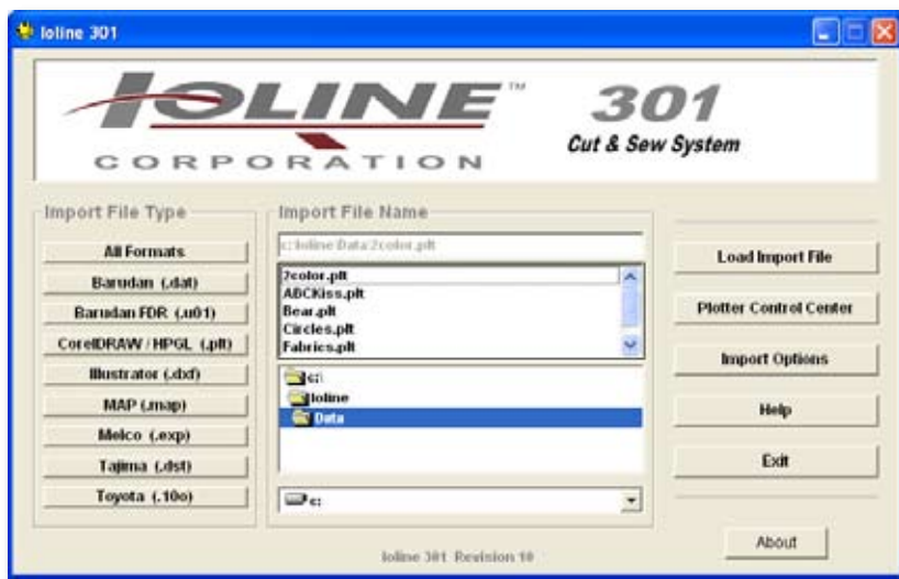
Figure 4. 301 Software icon.
